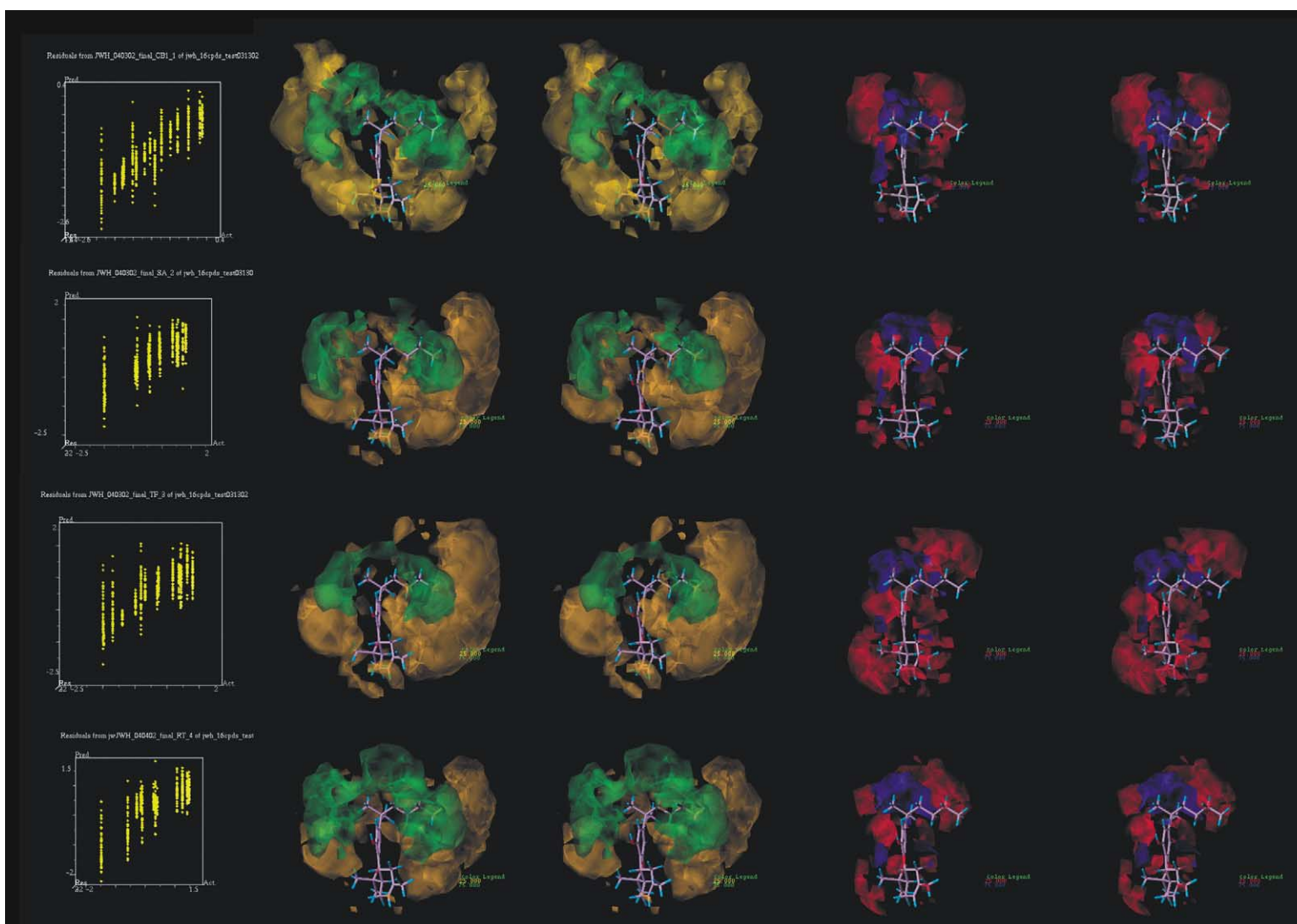
Figure 2. Predicted versus actual plots and stereoviews of the QSARS derived for the steric fields (yellow and green contours) and electrostatic fields (blue and red) as defined for cannabinoid receptor (CB1) binding affinity (A) and as defined for cannabinoid-induced changes in spontaneous locomotor activity (B), tail-flip latency (TF) and rectal temperature (RT). For each model, a 75/25 level of contribution is shown. The steric plots are depicted so that steric bulk should be moved closer to areas contoured in green and farther from regions in yellow in order to increase the target property being contoured (i.e., affinity or potency). The electrostatic plots are contoured such that positive charge should be moved closer to regions contoured in blue and farther from regions contoured in red in order to increase the target property being contoured.
